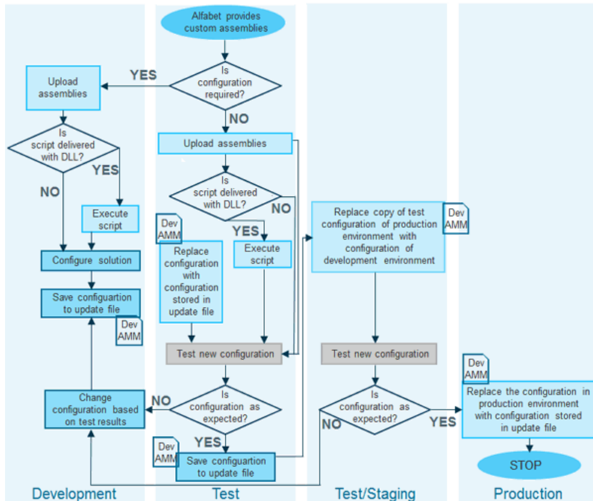
FIGURE: Example for a best practice workflow for the upload of custom assemblies to the database
