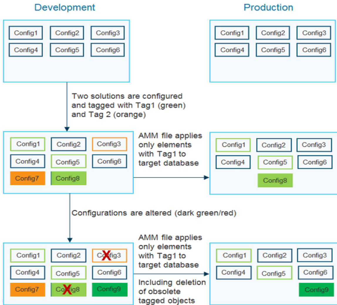
FIGURE: Configuration changes applied to a target database using solution tagging mechanisms in AMM files
