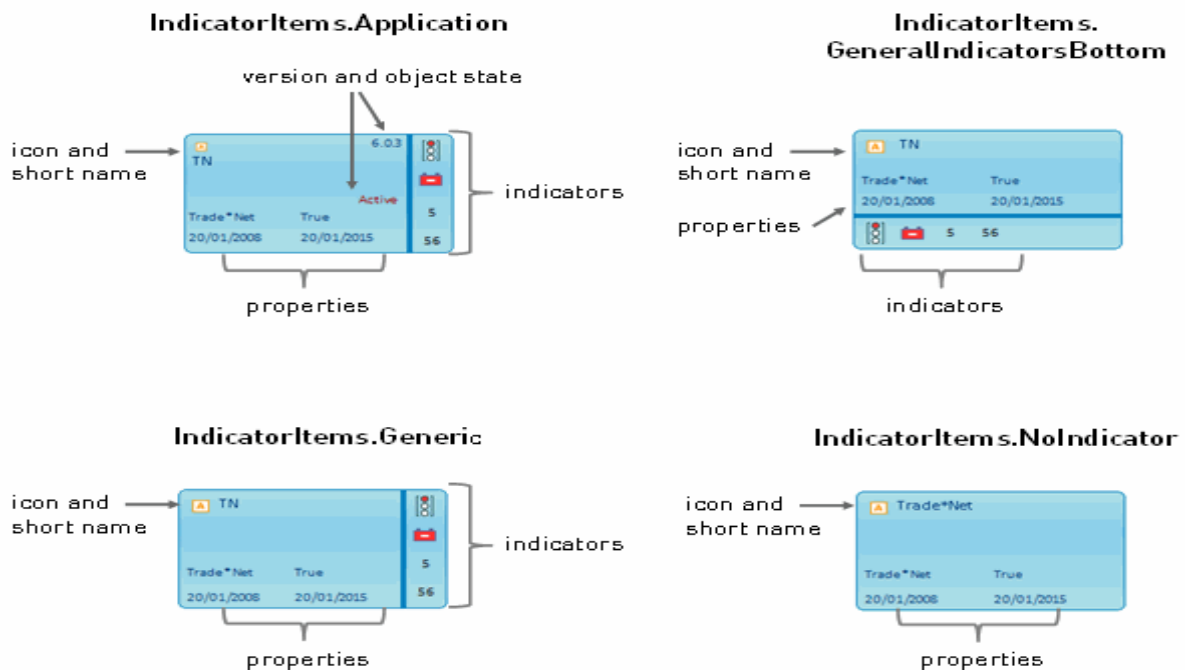
FIGURE: Standard diagram item templates available for architecture elements
