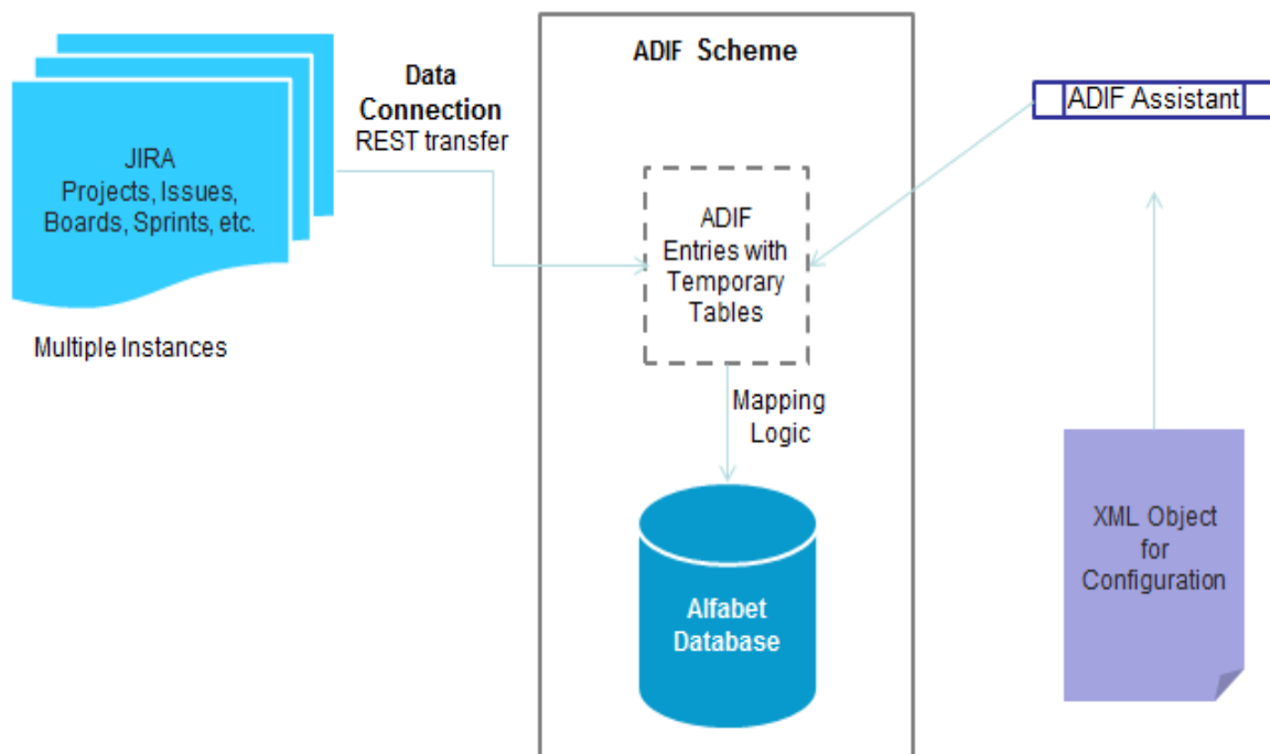
FIGURE: Overview of import from Jira
