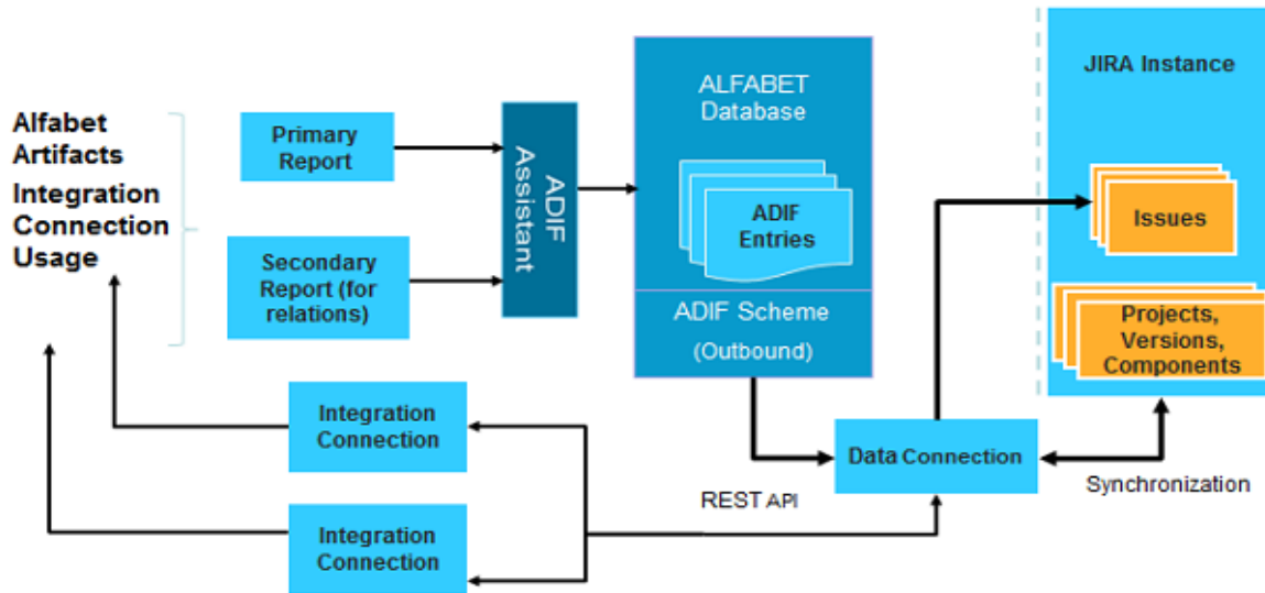
FIGURE: Overview of export to Jira
