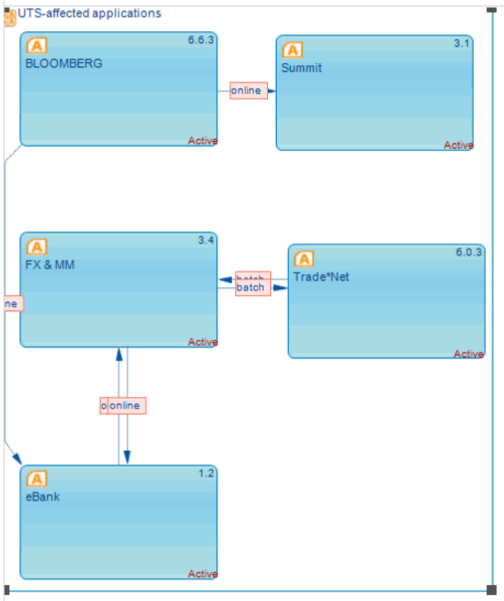
FIGURE: Information flows displaying Connection Type attributes in decoration boxes
