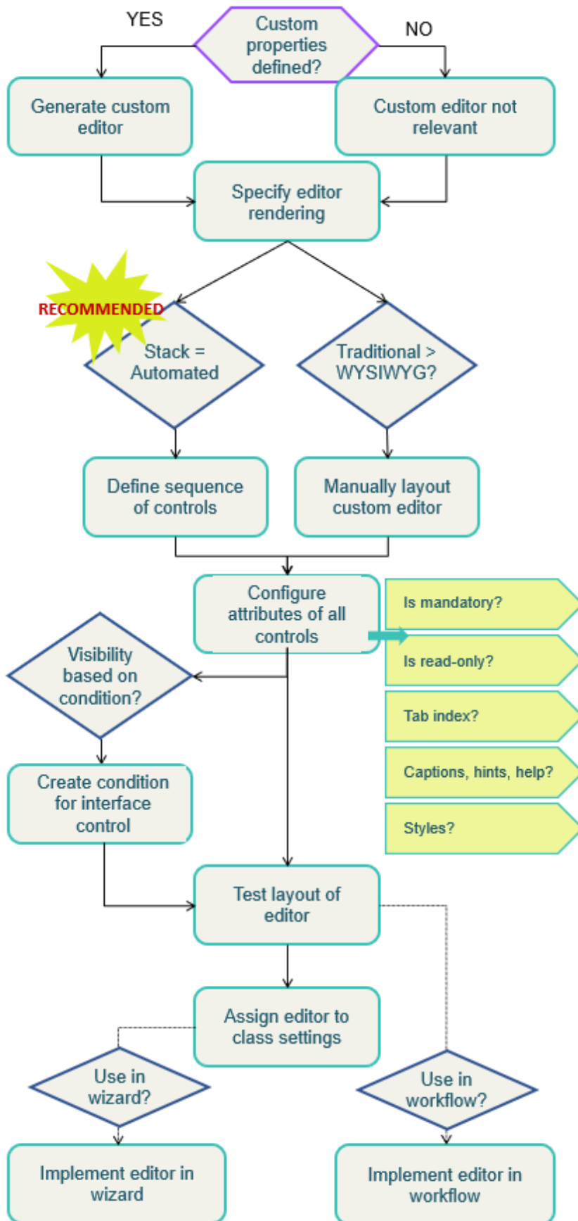
FIGURE: Steps to configure a custom editor
