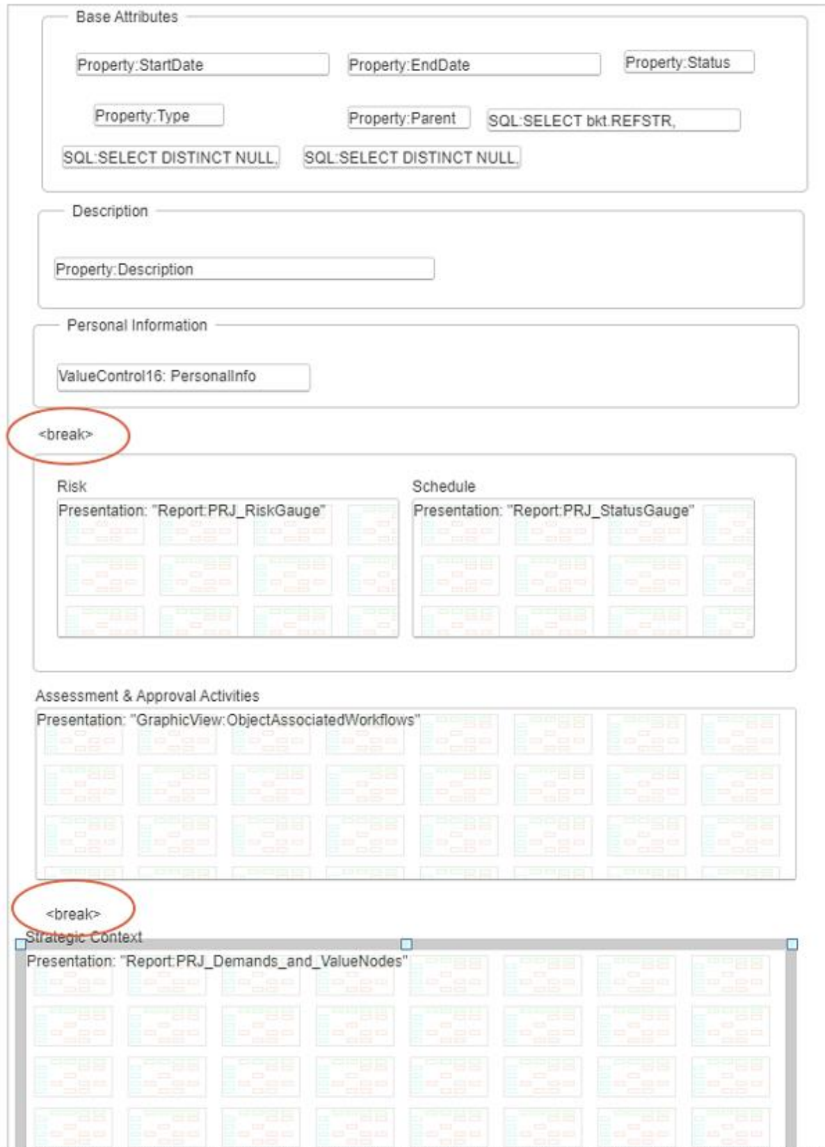
FIGURE: Configuration of line breaks
